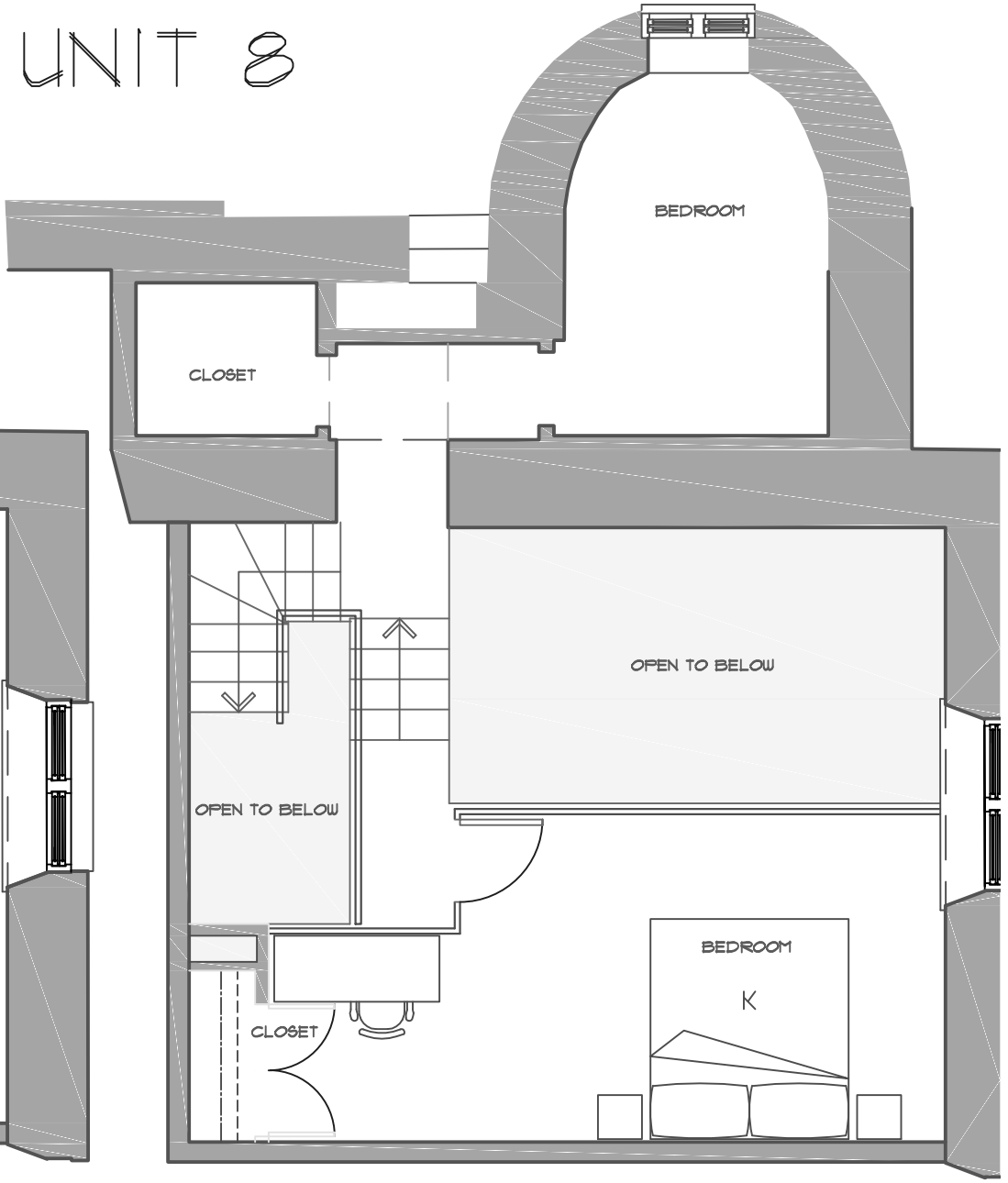
MEZZANINE
